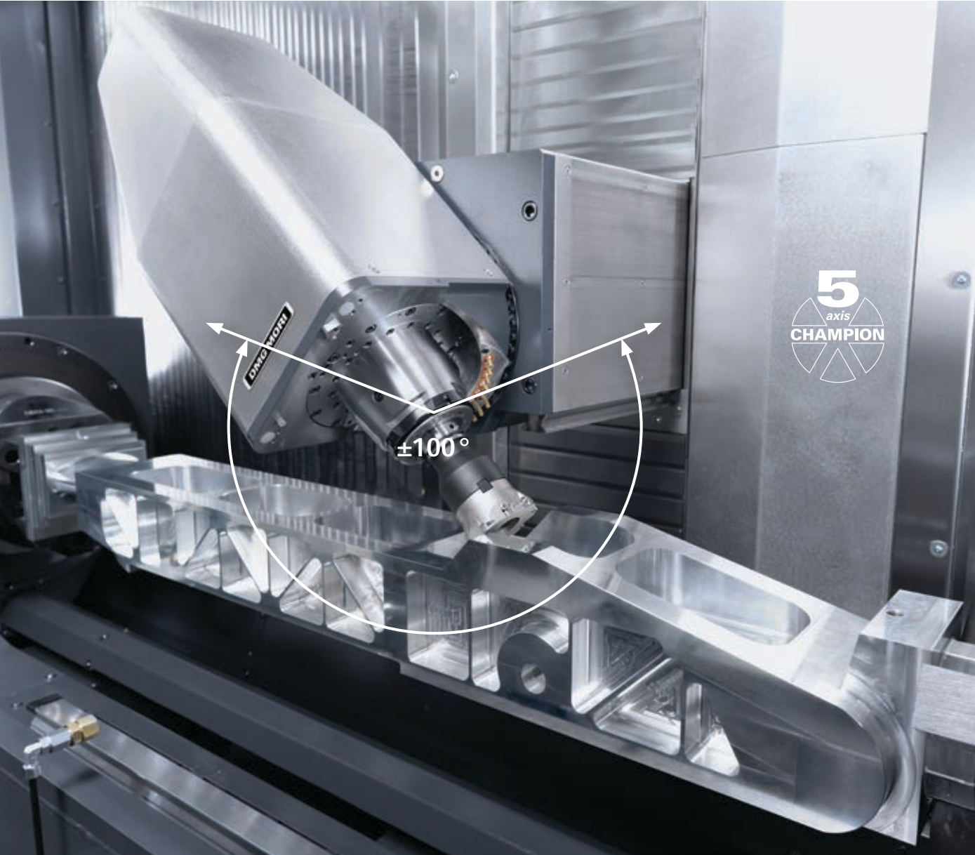
5-axis machining of a traverse on the DMF 260I7 with engineering racks.
