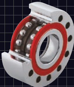
Ball Screw Support Unit (BSTU)
