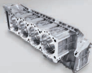
19.7 × 11.8 × 9.8 in. Crankcase / Automotive Material: Aluminum
