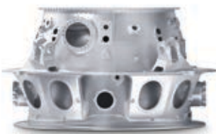
3 ø 59.1 × 29.5 in. Manifold DMU Portal FD Series Material: Titanium 6-4
