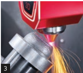
3 Combination laser metal deposition and milling on the LASERTEC 65 3D (flexible changing possible).
