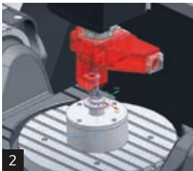
2 3D-simulation for collision monitoring with consideration of the built-in laser head.
