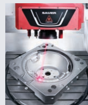
LASERTEC 65 Shape: 5-axis laser texturing / application of finish to a steering wheel mold.
